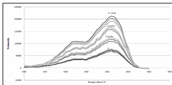
Fig 9: Glow curves of the unirradiated disks (N), the irradiated disks with 90 Sr beta radiation source at three different doses (N+10Gy, N+20Gy and N+30Gy), all for sample H1a.
