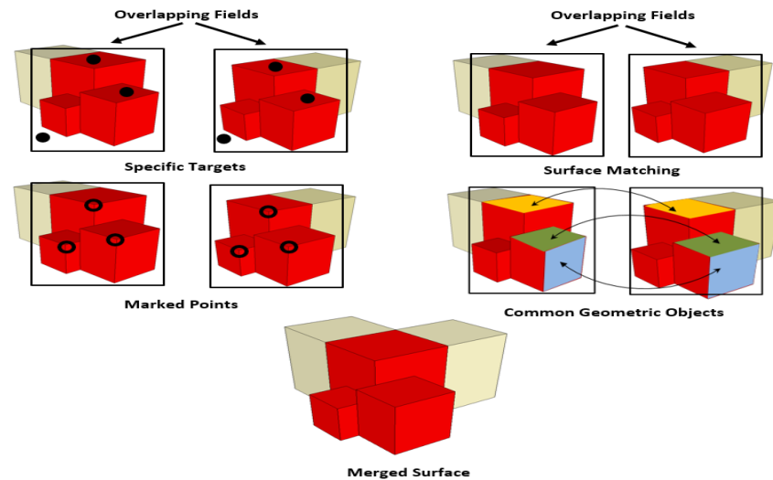
Figure 2. Registration approaches used in TLS applications
