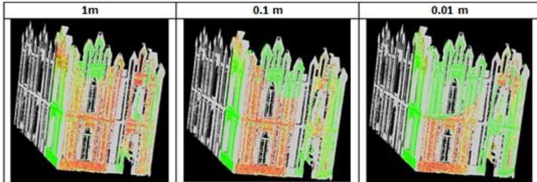
Figure 6. Surface-matching based on the distance between points
