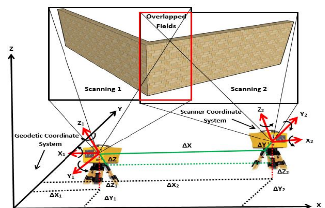
Figure 1. Registration of two scans
