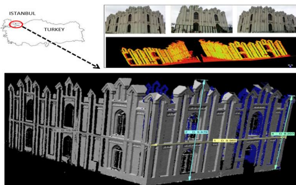
Figure 3. Image of the Historical Building Facade and Point Clouds
