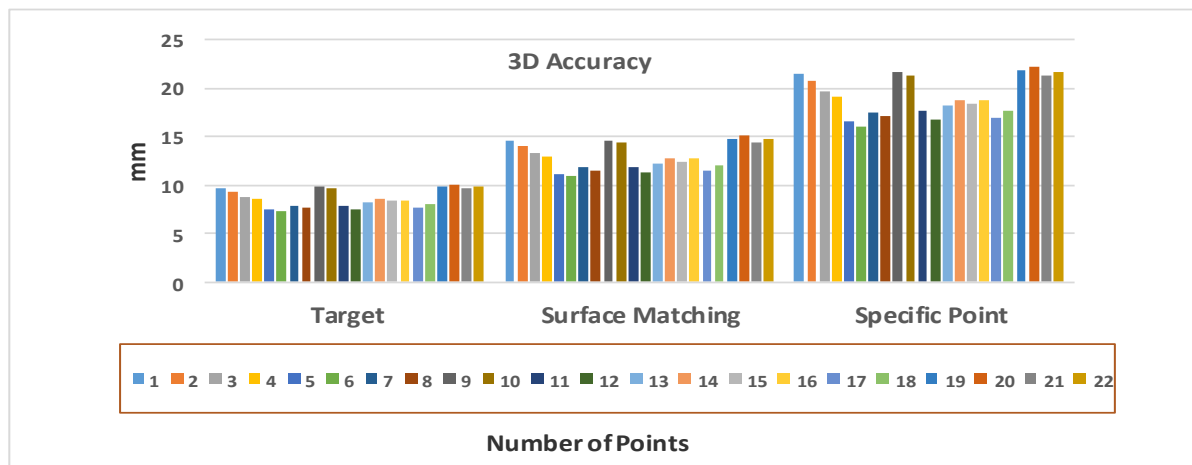
Figure 8. Weighted 3D positional accuracies (mm)
