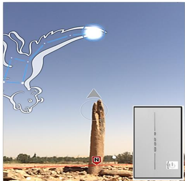
Figure 9. Simulation of the alignment found in group 1, using the software Skyview.
