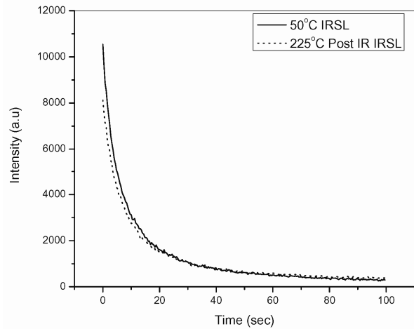
Fig. 6 Post IR IRSL SAR protocol for the dating of volcanic ash (following Buylaert et al. 2009).
