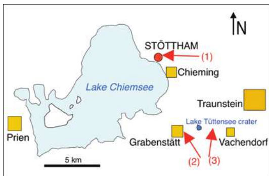
Figure 2. Location map for the Stöttham archaeological excavation (1) and the Grabenstätt (2) and Mühlbach (3) geologic excavations.
