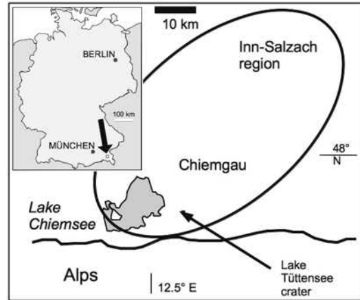
Figure 1. Location map for the Chiemgau region and the outline of the elliptically shaped strewn field of the Chiemgau impact event.
